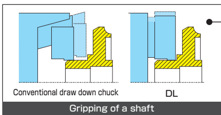
Gripping of a shaft
