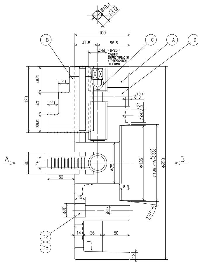
断面C-O-D SEC. C-O-D
